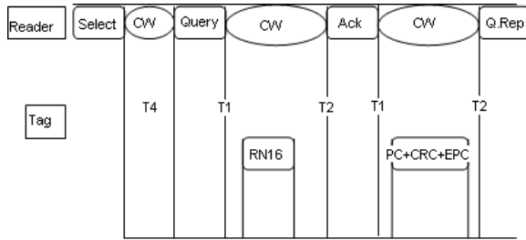
Figure 2: Generation 2 for Single tag reading
